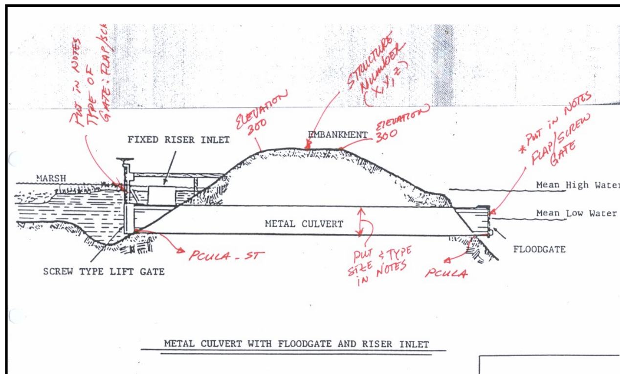
Figure 17: Basic Survey Coding For Culvert With Screw Gate And Flap Gate Inlets.
