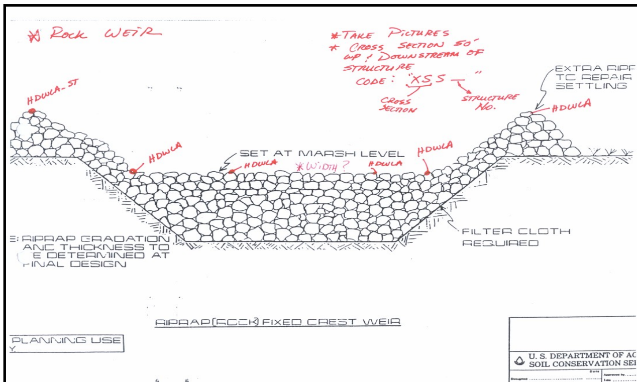
Figure 16: Basic Survey Coding For Rock Weir Structure
