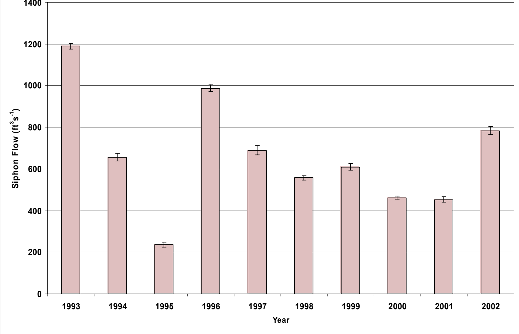
BA-04 Yearly Mean ( \pm SE) Siphon Flow ( \text{ft}^3 \text{s}^{-1} ) from 1993-2002
