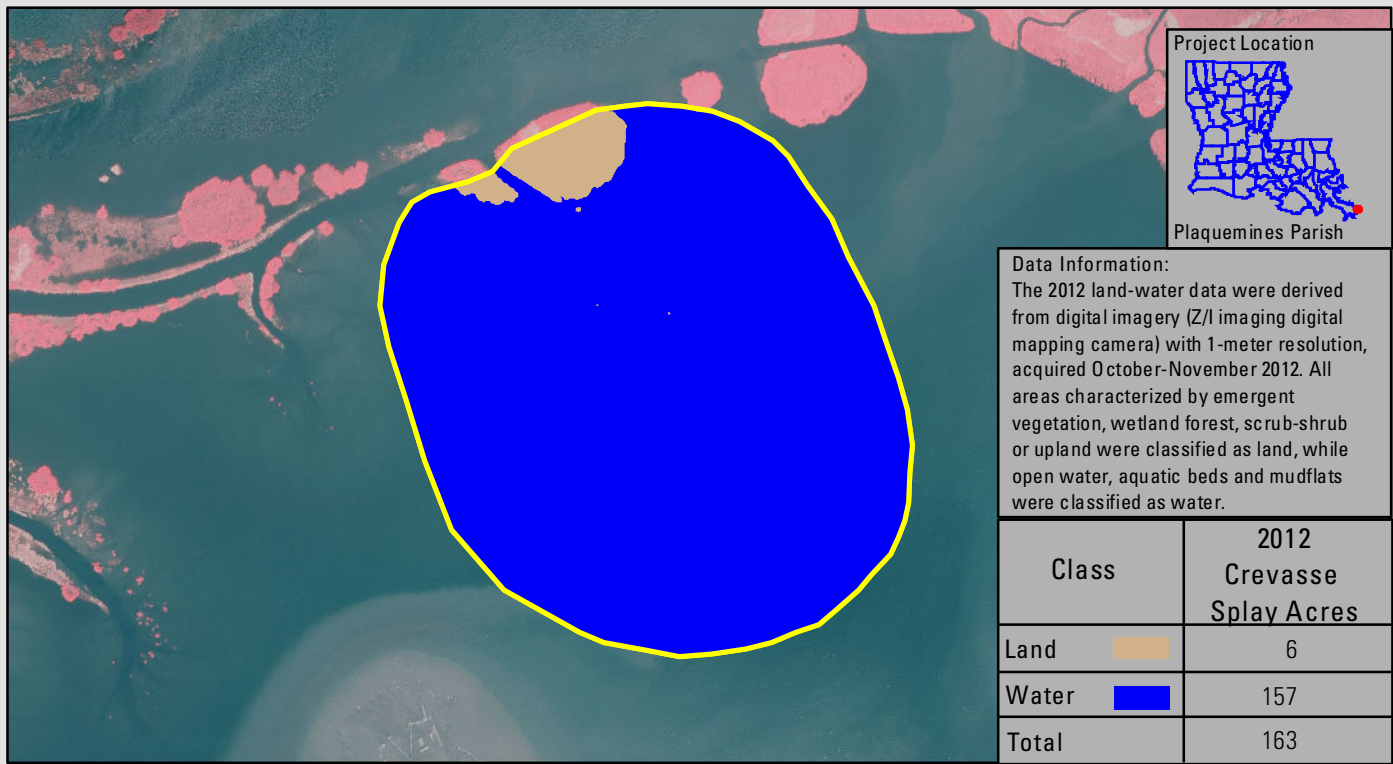
2012 Land-Water Classification
